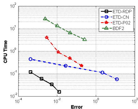
(c) Efficiency
