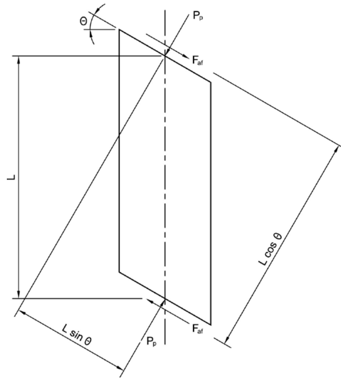
Figure 9. Soil pressure load, P_p , and soil/abutment interface friction, F_{af} .
