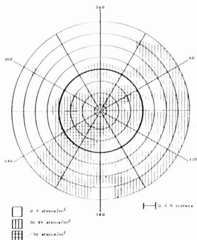
Fig. 1. Density (stems/meter 2 ) of sugar maple reproduction within 15 meters of maple. Approximate position of canopy dripline is indicated by heavy line.
