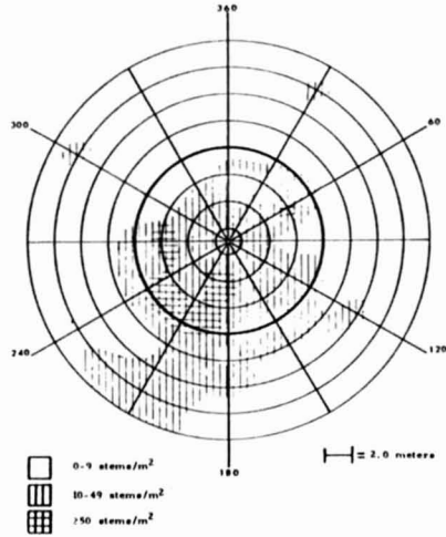
Fig. 2. Density (stems/m 2 ) of 2 year old sugar maple seedlings within 15 meters of maple. Approximate position of canopy dripline is indicated by heavy line.
