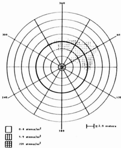
Fig. 3. Density (stems/m 2 ) of sugar maple reproduction older than 5 years. Approximate position of canopy dripline is indicated by heavy line.
