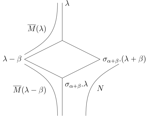
Figure 4.2: Submodule lattice when (\lambda + \rho, \beta) = 0 and (\lambda + \rho, (\alpha + \beta)^\vee) is integral.
