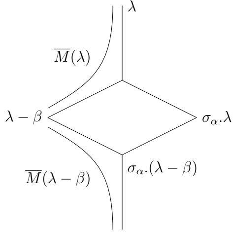
Figure 4.1: Submodule lattice when (\lambda + \rho, \beta) = 0 and (\lambda + \rho, \alpha^\vee) is integral.
