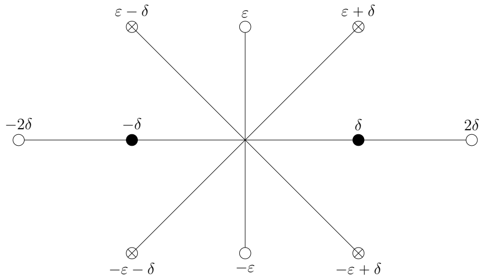
Figure 1.1: The root space of \mathfrak{osp}(3, 2)
