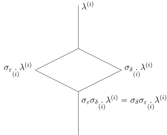
Figure 3.1: The structure of M = M^{(1)}(\lambda^{(1)}) = M^{(2)}(\lambda^{(2)}) when (\lambda^{(i)} + \rho^{(i)}, \varepsilon^\vee) \in \mathbb{N}^+ and (\lambda^{(i)} \rho^{(i)}, \delta^\vee) \in \mathbb{N}^{\text{odd}} .
