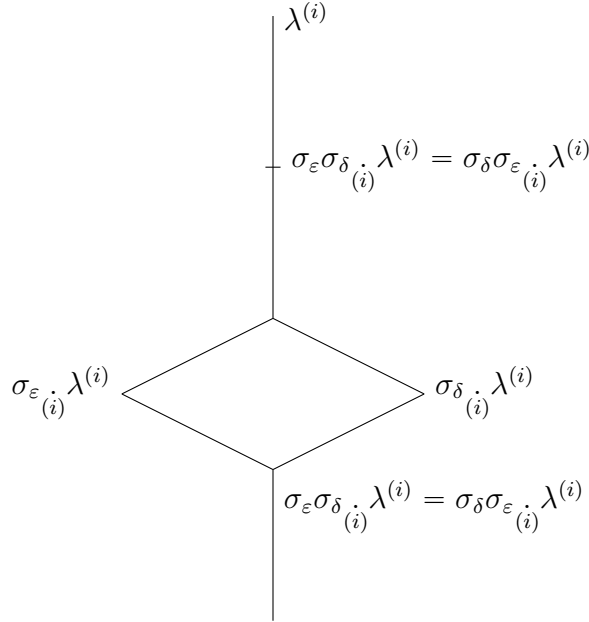
Figure 3.2: To show that the structure of M is that shown in fig. 3.1, we must eliminate this possibility.
