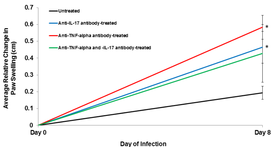
Figure 2. Overall change in paw swelling following treatment of B. burgdorferi -infected IL-10-deficient mice. Mice were infected with B. burgdorferi and then injected with antibodies to TNF- \alpha , IL-17, both cytokines, or neither cytokine for four days. Treatment with anti-TNF- \alpha or anti-IL-17 antibodies resulted in a significantly greater overall change in paw swelling compared to untreated controls. However, additional treatment with anti-TNF- \alpha did not result in swelling changes in anti-IL-17 antibody-treated mice. Values indicate means \pm SEM. Groups consisted of 4-5 mice each. *, P \geq 0.05 .
