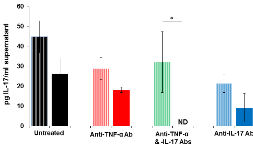
Figure 8. Effect of in vitro stimulation with B. burgdorferi for 24 hours on production of IL-17 from infected mice treated with anti-cytokine Abs. Stimulation with B. burgdorferi (darker bars) for 24 hours caused a decrease in IL-17 production by spleen cells obtained from infected mice treated with anti-cytokine Abs. A statistically significant decrease in IL-17 production was observed following stimulation of cells from dual-Ab-treated mice. Values indicate means \pm SEM. Groups consisted of 4-5 mice each. *, P \geq 0.05 .
