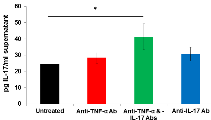
Figure 11. Production of IL-17 by B. burgdorferi -stimulated spleen cells from B. burgdorferi -infected, Ab-treated IL-10-deficient mice after 24 hours of incubation. Eight days after infection, spleen cells from Ab-treated, IL-10-deficient mice were incubated for 24 hours in the presence of B. burgdorferi . Cells from anti-TNF- \alpha Ab-treated mice produced a similar amount of IL-17 as cells from untreated mice. Although the amount of IL-17 produced by cells of dual-Ab-treated mice was significantly greater than controls, it was similar to that of cells from anti-IL-17 Ab-treated mice. Values indicate means \pm SEM. Groups consisted of 4-5 mice each. *, P \geq 0.05 .
