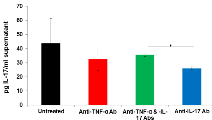
Figure 13. Effect of 5 \mu g in vitro anti-cytokine Abs on production of IL-17 in wild-type cells. Wild-type mice were infected with B. burgdorferi . Eight days later, spleen cells were incubated with 5 \mu g of anti-TNF- \alpha Ab, anti-IL-17 Ab, or both Abs for 24 hours. Anti-TNF- \alpha Ab treatment of IL-17 Ab-treated cells caused a significant increase in IL-17 production compared to cells treated with anti-IL-17 Ab alone. Values indicate means \pm SEM. Groups consisted of 4-5 mice each. *, P \geq 0.05 .
