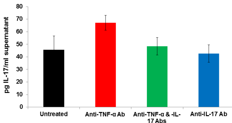
Figure 4. Production of IL-17 by B. burgdorferi -stimulated spleen cells from B. burgdorferi -infected, Ab-treated wild-type mice after 18 hours of incubation. Eight days after infection, spleen cells from Ab-treated, wild-type mice were incubated for 18 hours in the presence of B. burgdorferi . Stimulated cells from anti-TNF- \alpha Ab-treated mice produced slightly, but not significantly, more IL-17 than stimulated cells from untreated, infected mice. Anti-TNF- \alpha Ab treatment did not affect IL-17 production by cells from mice treated with anti-IL-17 Abs. Values indicate means \pm SEM. Groups consisted of 4-5 mice each.
