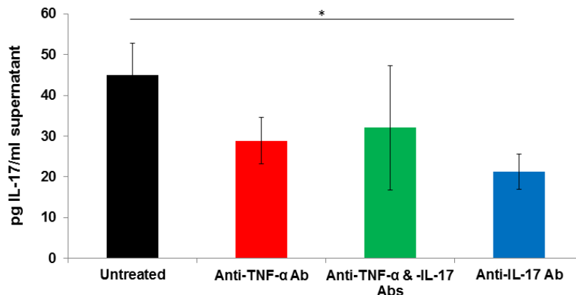
Figure 6. Production of IL-17 by unstimulated spleen cells from B. burgdorferi -infected, Ab-treated wild-type mice after 24 hours of incubation. Eight days after infection, spleen cells from Ab-treated, wild-type mice were incubated for 24 hours in the absence of B. burgdorferi . Unstimulated cells from anti-TNF- \alpha Ab-treated mice produced a similar amount of IL-17 than unstimulated cells from untreated, infected mice. By contrast, cells from anti-IL-17 Ab-treated mice produced significantly less IL-17 than cells from control mice. The level of IL-17 produced by cells from anti-IL-17 Ab-treated mice was comparable to that of cells from anti-IL-17 and -TNF \alpha Ab-treated mice. Values indicate means \pm SEM. Groups consisted of 4-5 mice each. *, P \geq 0.05 .
