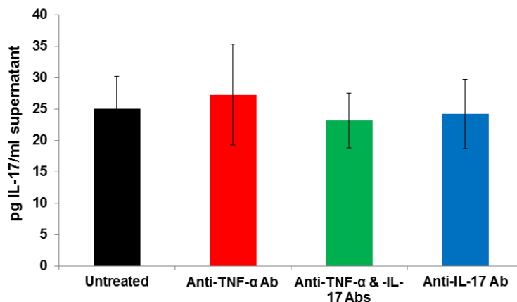
Figure 10. Production of IL-17 by unstimulated spleen cells from B. burgdorferi -infected, Ab-treated IL-10-deficient mice after 24 hours of incubation. Eight days after infection, spleen cells from Ab-treated, IL-10-deficient mice were incubated for 24 hours in the absence of B. burgdorferi . No differences in IL-17 production were observed among cells from any of the Ab-treated mice. Values indicate means \pm SEM. Groups consisted of 4-5 mice each.
