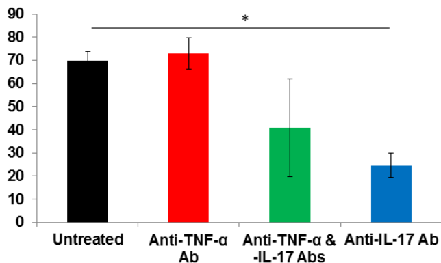
Figure 17. Effect of 10 µg in vitro anti-cytokine Abs on production of IL-17 in IL-10-deficient cells. IL-10-deficient mice were infected with B. burgdorferi . Eight days later, spleen cells were incubated with 10 µg of anti-TNF-α Ab, anti-IL-17 Ab, or both anti-TNF-α and anti-IL-17 Ab for 24 hours. Cells treated with anti-IL-17 Ab produced significantly less IL-17 than untreated cells. Cells treated with anti-TNF-α Ab alone, or in addition to anti-IL-17 Ab, had no effect on IL-17 production. Values indicate means ± SEM. Groups consisted of 4-5 mice each. *, P \geq 0.05 .
