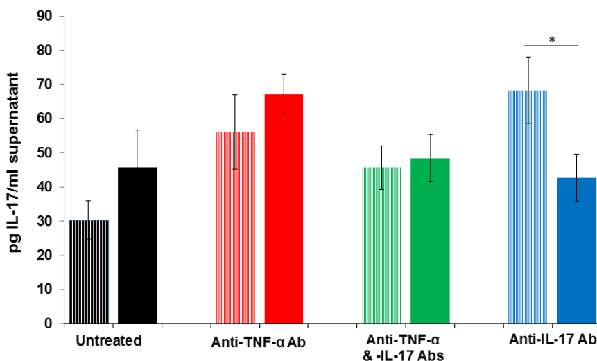
Figure 5. Effect of in vitro stimulation with B. burgdorferi for 18 hours on production of IL-17 from infected mice treated with anti-cytokine Abs. Stimulation with B. burgdorferi (darker bars) caused a slight, but insignificant, increase in IL-17 production by spleen cells obtained from infected mice that were untreated or treated with anti-TNF- \alpha Abs. By contrast, stimulation caused a significant decrease in IL-17 production by cells obtained from infected mice treated with anti-IL-17 Abs. Values indicate means \pm SEM. Groups consisted of 4-5 mice each. *, P \geq 0.05 .
