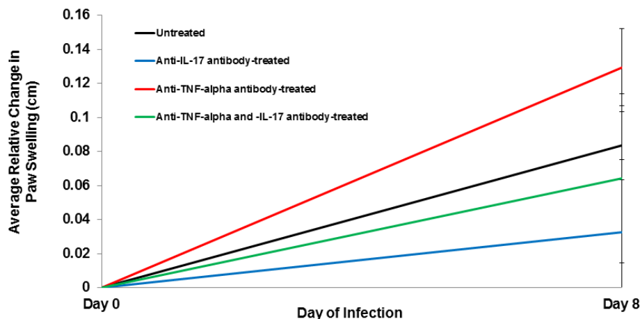
Figure 1. Overall change in paw swelling following treatment of B. burgdorferi -infected wild-type mice. Mice were infected with B. burgdorferi and then injected with antibodies to TNF- \alpha , IL-17, both cytokines, or neither cytokine for four days. Treatment with TNF- \alpha antibodies slightly, but not significantly, increased paw swelling in mice that were otherwise not treated or treated with anti-IL-17 antibodies. Values indicate means \pm SEM. Groups consisted of 4-5 mice each.
