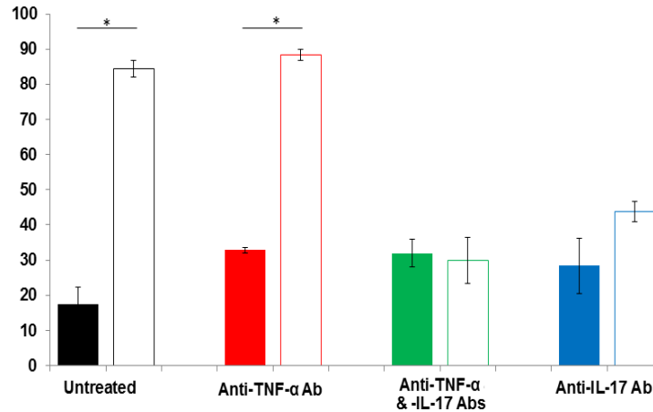
Figure 18. Effect of IL-10 deficiency on IL-17 production. Untreated or anti-TNF- \alpha Ab-treated cells from IL-10-deficient mice (open bars) produce significantly more IL-17 than wild-type counterparts (closed bars) when incubated with 2.5 \mu g Ab. No difference in IL-17 production was observed when cultures contained anti-IL-17 antibody. Values indicate means \pm SEM. Groups consisted of 4-5 mice each. *, P \geq 0.05 .
