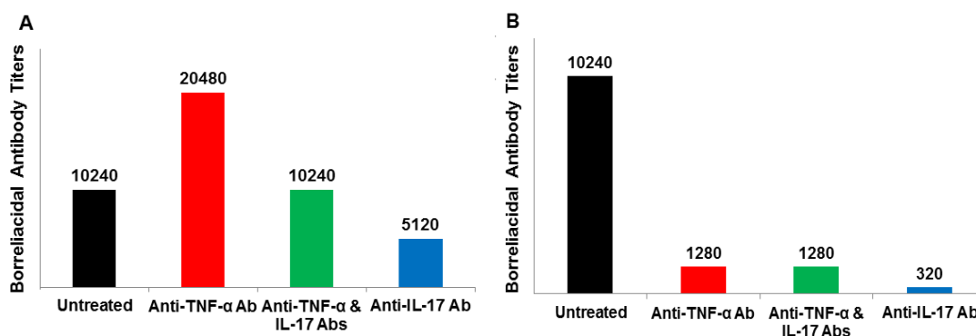
Figure 19. Borreliacidal antibody production. Borreliacidal antibody titers from serum of wild-type (A) and IL-10-deficient (B) mice. Mice were infected with B. burgdorferi and were untreated or treated with anti-TNF- \alpha Ab, anti-IL-17 Ab, or both anti-TNF- \alpha and anti-IL-17 Abs for 4 days following infection. Sera were collected on day 8 after infection. Groups consisted of 4-5 mice each.
