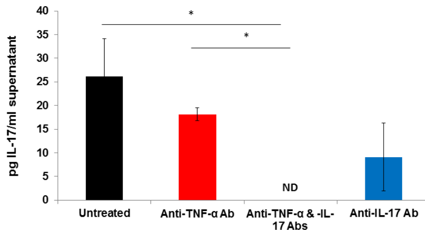
Figure 7. Production of IL-17 by B. burgdorferi -stimulated spleen cells from B. burgdorferi -infected, Ab-treated wild-type mice after 24 hours of incubation. Eight days after infection, spleen cells from Ab-treated, wild-type mice were incubated for 24 hours in the presence of B. burgdorferi . Stimulated cells from anti-TNF- \alpha and anti-IL-17 Ab-treated mice produced a similar amount of IL-17 as unstimulated cells from untreated, infected mice. By contrast, cells from dual-Ab-treated mice produced undetectable amounts of IL-17. While this was significantly less compared to cells of untreated or anti-TNF- \alpha Ab-treated mice, it was not significantly different compared to cells of IL-17 Ab-treated mice. Values indicate means \pm SEM. Groups consisted of 4-5 mice each. *, P \geq 0.05 .
