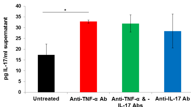
Figure 12. Effect of 2.5 \mu g in vitro anti-cytokine Abs on production of IL-17 in wild-type cells. Wild-type mice were infected with B. burgdorferi . Eight days later, spleen cells were incubated with 2.5 \mu g of anti-TNF- \alpha Ab, anti-IL-17 Ab, or both anti-TNF- \alpha and anti-IL-17 Ab for 24 hours. Cells treated with anti-TNF- \alpha Ab produced significantly more IL-17 than untreated cells. However, anti-TNF- \alpha Ab treatment did not affect IL-17 production by cells treated with anti-IL-17 Ab. Values indicate means \pm SEM. Groups consisted of 4-5 mice each. *, P \geq 0.05 .
