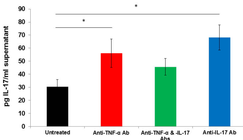
Figure 3. Production of IL-17 by unstimulated spleen cells from B. burgdorferi -infected, antibody (Ab)-treated wild-type mice after 18 hours of incubation. Eight days after infection, spleen cells from Ab-treated, wild-type mice were incubated for 18 hours in the absence of B. burgdorferi . Unstimulated cells from anti-TNF- \alpha and anti-IL-17 Ab-treated mice produced significantly more IL-17 than unstimulated cells from untreated, infected mice. Additional treatment with anti-TNF- \alpha Ab did not affect IL-17 production by cells of anti-IL-17 Ab-treated mice. Values indicate means \pm SEM. Groups consisted of 4-5 mice each. *, P \geq 0.05 .
