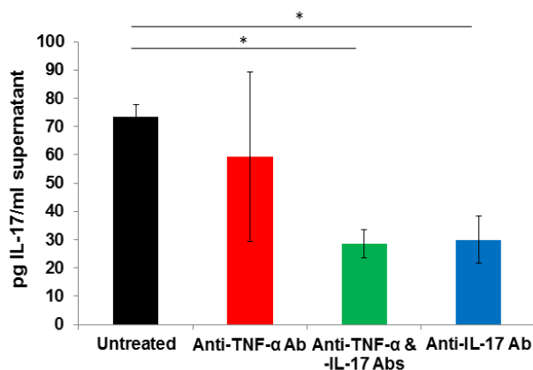
Figure 16. Effect of 5 µg in vitro anti-cytokine Abs on production of IL-17 in IL-10-deficient cells. IL-10-deficient mice were infected with B. burgdorferi . Eight days later, spleen cells were incubated with 5 µg of anti-TNF-α Ab, anti-IL-17 Ab, or both anti-TNF-α and anti-IL-17 Ab for 24 hours. Cells treated with anti-IL-17 Ab, with or without anti-TNF-α Ab, produced significantly less IL-17 than untreated cells. Cells treated with anti-TNF-α Ab alone had no effect on IL-17 production. Values indicate means ± SEM. Groups consisted of 4-5 mice each. *, P \geq 0.05 .
