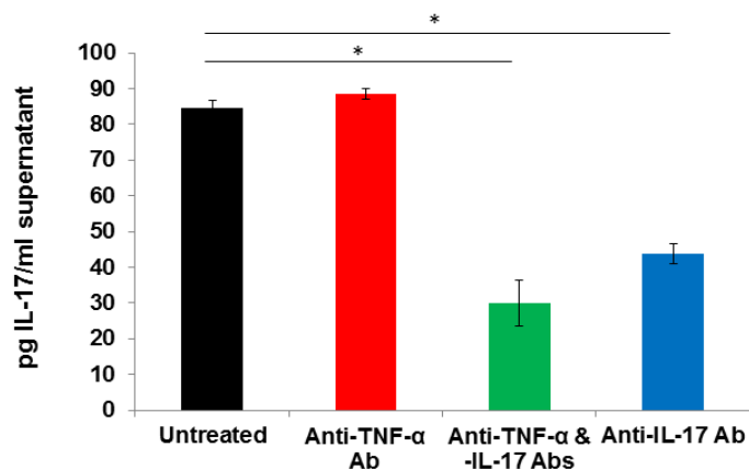
Figure 15. Effect of 2.5 µg in vitro anti-cytokine Abs on production of IL-17 in IL-10-deficient cells. IL-10-deficient mice were infected with B. burgdorferi . Eight days later, spleen cells were incubated with 2.5 µg of anti-TNF-α Ab, anti-IL-17 Ab, or both anti-TNF-α and anti-IL-17 Ab for 24 hours. Cells treated with anti-IL-17 Ab produced significantly less IL-17 than untreated cells, but cells treated with anti-TNF-α Ab alone had no effect. Anti-TNF-α Ab treatment did not affect IL-17 production by cells also treated with anti-IL-17 Ab. Values indicate means ± SEM. Groups consisted of 4-5 mice each. *, P ≥ 0.05.
