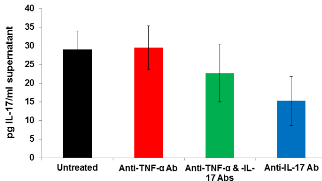
Figure 14. Effect of 10 µg in vitro anti-cytokine Abs on production of IL-17 in wild-type cells. Wild-type mice were infected with B. burgdorferi . Eight days later, spleen cells were incubated with 10 µg of anti-TNF-α Ab, anti-IL-17 Ab, or both anti-TNF-α and anti-IL-17 Ab for 24 hours. Anti-TNF-α Ab treatment had no effect on IL-17 production at this concentration. Values indicate means ± SEM. Groups consisted of 4-5 mice each. *, P \geq 0.05 .
