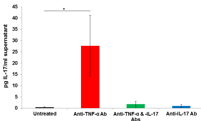
Figure 9. Production of IL-17 by B. burgdorferi -stimulated spleen cells from B. burgdorferi -infected, Ab-treated IL-10-deficient mice after 18 hours of incubation. Eight days after infection, spleen cells from Ab-treated, IL-10-deficient mice were incubated for 18 hours in the presence of B. burgdorferi . Stimulated cells from anti-TNF- \alpha Ab-treated mice produced significantly, more IL-17 than stimulated cells from untreated, infected mice. Values indicate means \pm SEM. Groups consisted of 4-5 mice each. *, P \geq 0.05 .
