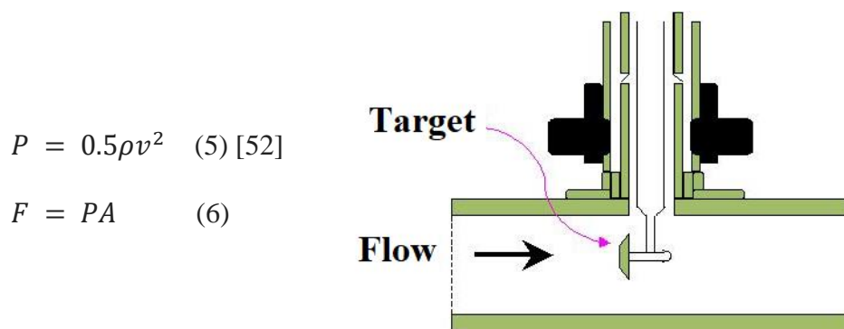
Figure 1- Target flow meter
