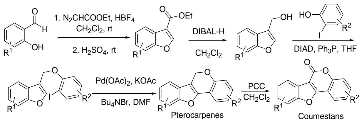
Scheme 3.21: Synthesis of Pterocarpenes and Coumestans
